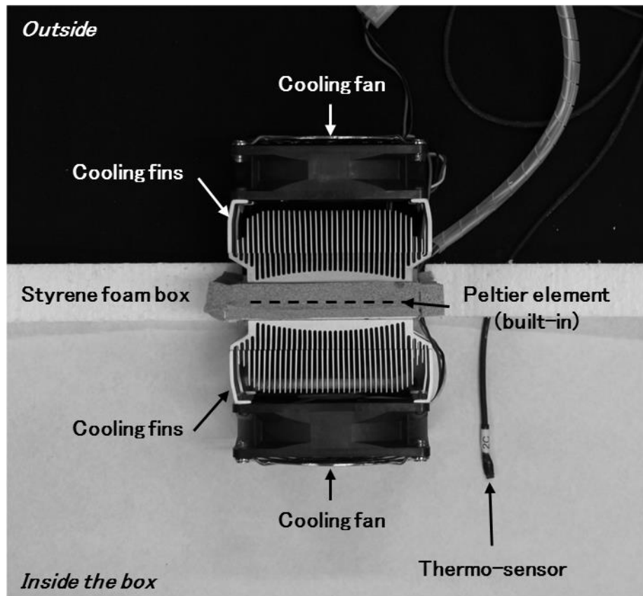
Fig. 3.1 A temperature control device applying thermoelectric cooling/heating element using Peltier effect. The Peltier element is sandwiched by two cooling-fin holders mounted with fans. The device is attached on a styrene foam box and can regulate the temperatures inside the box precisely without following outside-temperature fluctuation: device is governed by the Proportional-Integral-Derivative (PID) algorithm to keep a target temperature \pm 0.2^{\circ}\text{C} .
