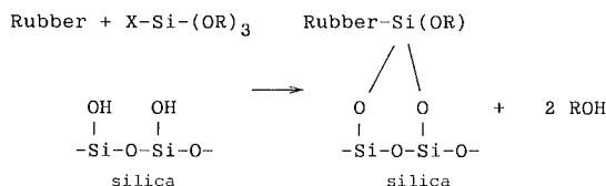
Figure 1. Reaction scheme of silane coupling agent for rubber/silica composite. X = NH 2 , CH 2 = CH, SH, epoxy etc.
