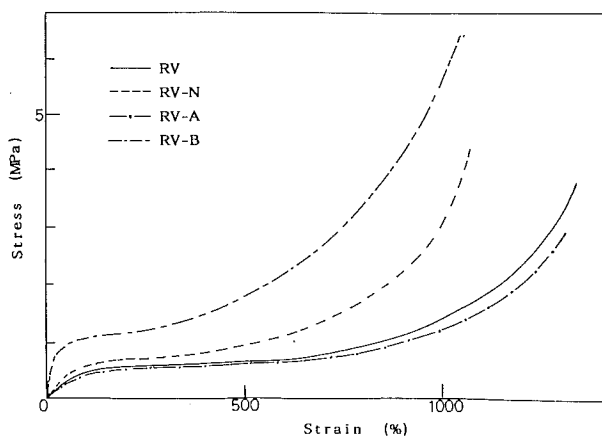
Figure 7. Tensile stress-strain curves of SBR vulcanizates with or without in situ silica.
