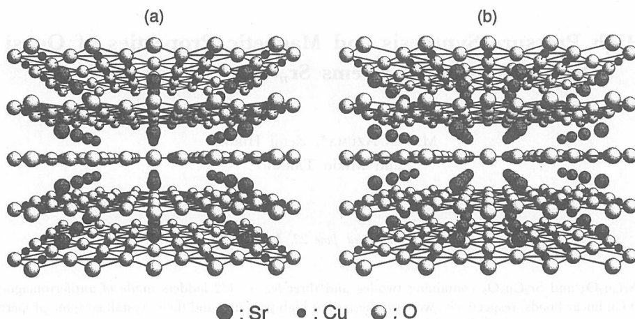
Fig. 1. \text{SrCu}_2\text{O}_3 (a) and \text{Sr}_2\text{Cu}_3\text{O}_5 (b).
