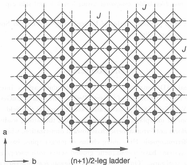
Fig. 2. Schematic drawing of the \text{Cu}_{n+1}\text{O}_{2n} sheet of \text{Sr}_{n-1}\text{Cu}_{n+1}\text{O}_{2n} . The filled circles are \text{Cu}^{2+} ions, and \text{O}^{2-} ions exist at the corners of the squares drawn with solid lines.
