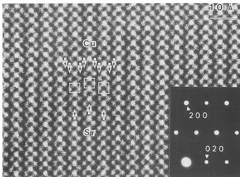
Fig. 4. High resolution electron microscopic images and the corresponding Electron diffraction patterns (inset) of \text{SrCu}_2\text{O}_3 along the c -axis.
