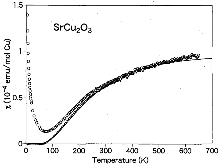
Fig. 6. Temperature dependence of the magnetic susceptibility of \text{SrCu}_2\text{O}_3 . The open circles are the experimental raw data, while the data after subtraction of the Curie component and the small orbital contribution are given with the dark dots. Solid line stands for the calculated susceptibility assuming the spin gap of 420 K using an equation \chi(T) \propto T^{-1/2} \exp(-\Delta/T) given in Ref. 10 (see text).
