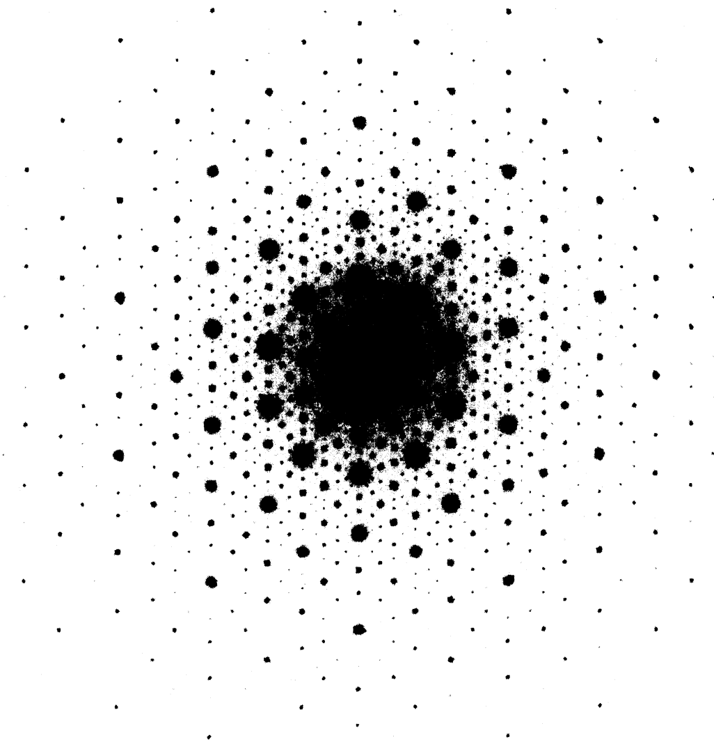
FIGURE 1. Experimental diffraction pattern of an icosahedral AlMnPd quasicrystal along the fivefold direction (courtesy C. Beeli).
