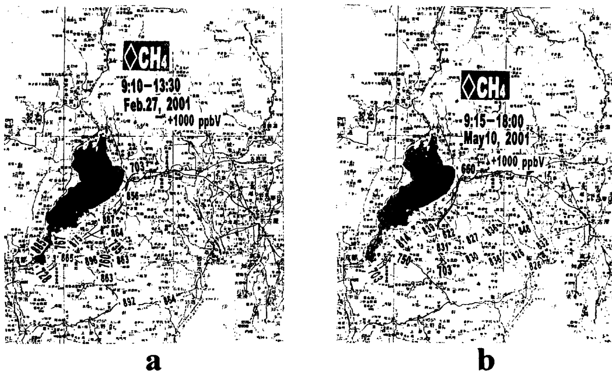
Fig. 2 Observation of atmospheric methane concentration in the southeastern part of Shiga-ken:
