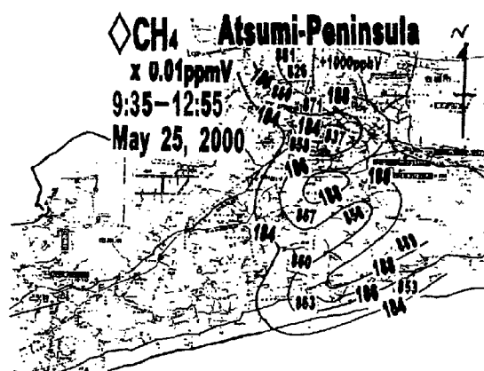
Fig.2-1 Spatial distribution of atmospheric CH 4 over the Atsumi Peninsula for 9:35-12:55 May 25, 2000
