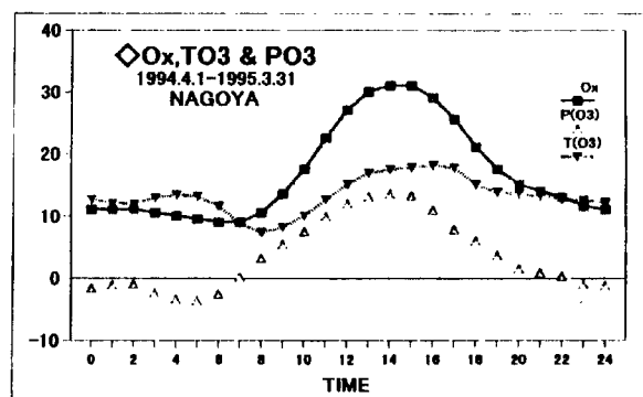
Fig.1-3 O_x , T(O_3) and their difference [P(O_3)] ( \equiv [O_x] - [T(O_3)] )
