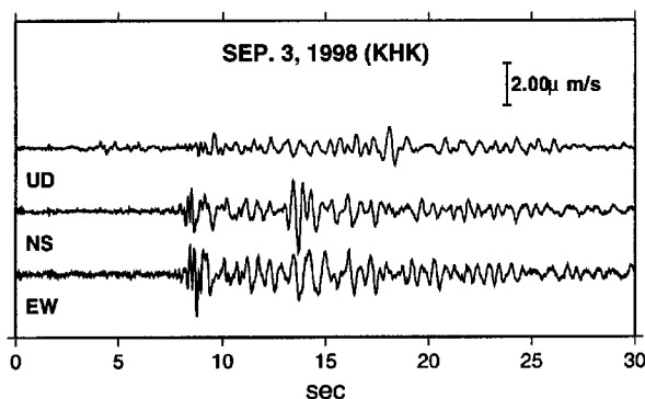
Fig. 14 An example of three components waveform of a DLF at the Mitoko fault system observed at station KHK.
