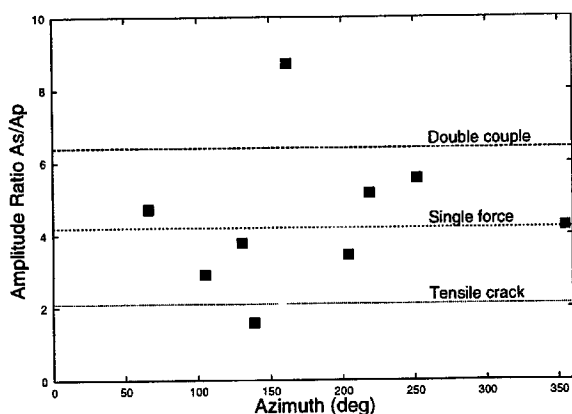
Fig. 7 The amplitude ratios of the S-waves to the P-waves as a function of azimuth for the DLF event shown in Fig.2(b). Seismograms recorded at Hi-net stations, which are installed at the bottom of 100 - 200 m boreholes, were used.
