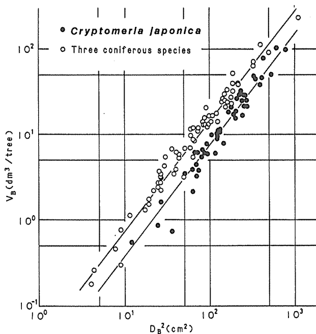
Fig. 6 Allometric relation between V_B and D_B^2 in individuals in Cryptomeria and the other three conifers. Values of V_B are obtained from Eqs. 6, 7. Branch weight ( w_B ) may be estimated by the specific gravity of the stems.
