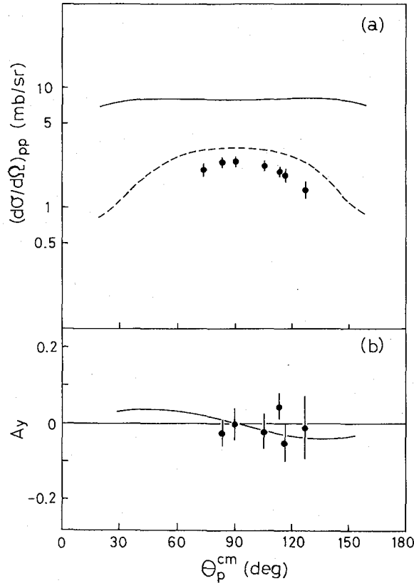
Fig. 3 Two-body pp cross sections deduced from observed QFS cross sections using the PWIA formula (a) and pp -QFS analyzing powers (b) for the {}^3\text{He}(\vec{p}, 2p){}^2\text{H} reaction at 64.9 MeV. Solid lines represent the pp elastic scattering cross section and analyzing power, and dashed line the elastic cross section multiplied by the MS factor.
