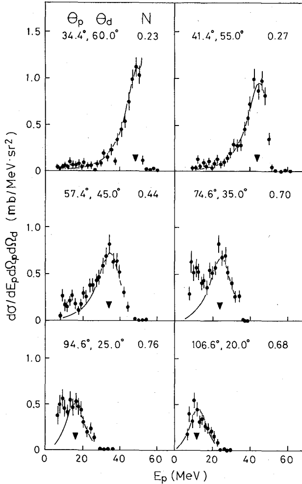
Fig. 2. Coincidence energy spectra for the {}^3\text{He}(\vec{p}, pd){}^1\text{H} reaction at 64.9 MeV. Solid lines represent the PWIA values multiplied by factors N .
