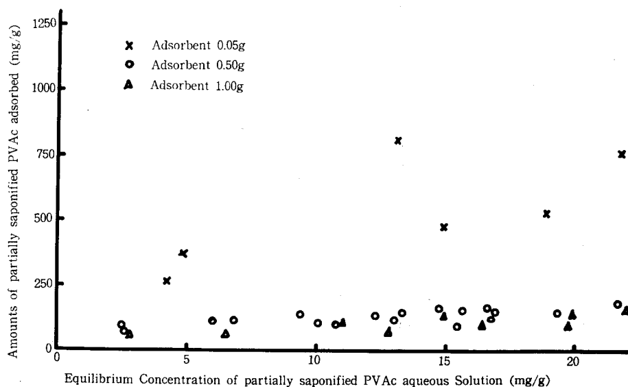
Fig. 4 Effects of the amounts of adsorbent (wood) added on the partially saponified PVAc adsorption. Amount of adsorbent are 0.05, 0.50 and 1.0 g., and on each case, the adsorption isotherms are determined separately.
