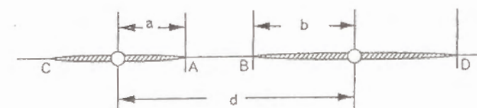
Fig. 4.1. Collinear cracks.
