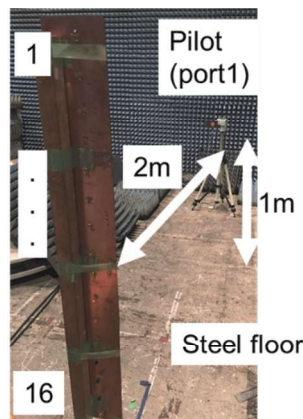
Fig.3. Experimental setup of multi-pass retrodirective
