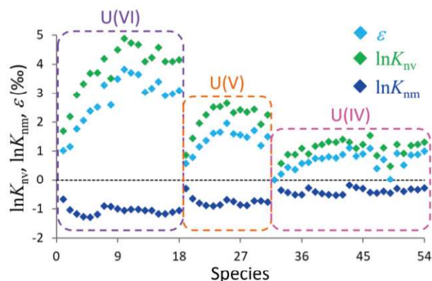
Fig. 1. \ln K_{nv} , \ln K_{nm} , and \varepsilon of 54 U species. The light blue, green, and deep blue plots represent \varepsilon , \ln K_{nv} , and \ln K_{nm} , respectively. These plots for U(VI), U(V), and U(IV) species are surrounded by the purple, orange, and pink rounded squares, respectively. [6]
