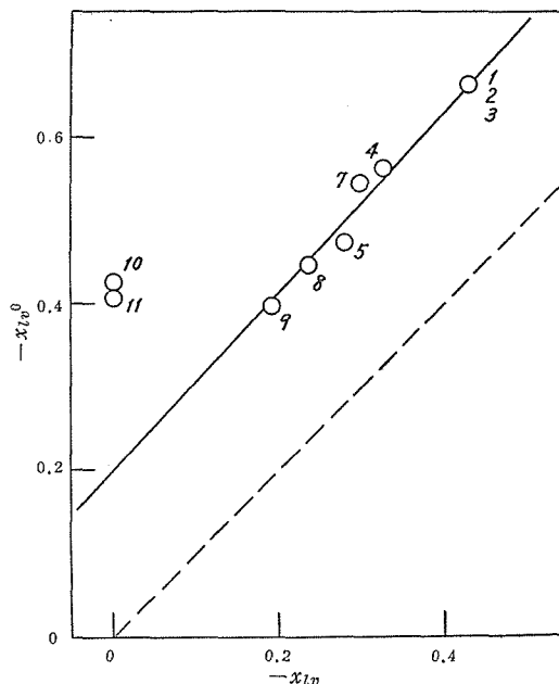
Fig. 2. Relation between x_{lv} and x_{lv}^0 of aromatic ketones. The broken line represents the relationship: x_{lv} = x_{lv}^0 . As to the numbering, see Table 1.
