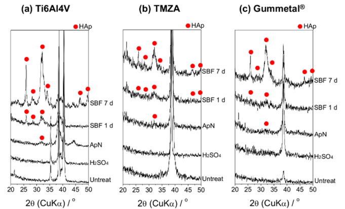
Fig. 5. XRD profiles of the surfaces of the untreated, H_2SO_4 -treated and subsequent ApN-treated (a) Ti6Al4V, (b) TMZA and (c) Gummetal ® specimens and those after the soak in the conventional SBF for 1 day and 7 days
