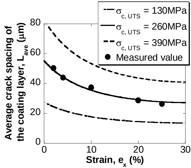
Fig.4.3 Measured average crack spacing L_{ave} in the coating layer with applied nominal strain [14], together with the predicted changes of L_{ave} for weak ( \sigma_{c, UTS} = 130 MPa ) and strong (390MPa) coating layer.
