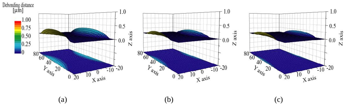
Fig.7.6 Calculated distributions of the interfacial debonding distance from the substrate to coat (i) at 5% tensile strain in the x-direction under the condition of \sigma_{(i), \text{int.}} = 100\text{MPa} and \sigma_{(ii), \text{int.}} = (a) 60MPa, (b) 80MPa and (c) 100MPa.
