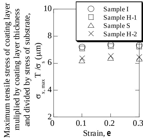
Fig.3.5 Relation between \sigma_{x, \max} T / \sigma_c (the maximum tensile stress of coating layer multiplied by the coating layer thickness and divided by the stress of substrate) to the nominal strain e . (Coating layer thickness T = 10\mu\text{m} for Samples I and H-1, and T = 5\mu\text{m} for Samples S and H-2. Crack spacing L = 40\mu\text{m} .)
