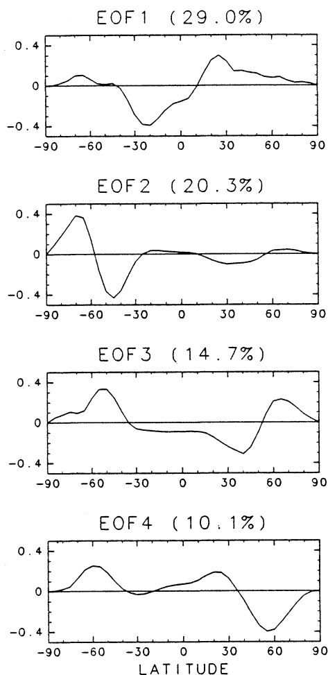
Fig. 2. The first four EOF profiles of [Z_s] . Contribution to the total variance is written in parentheses.
