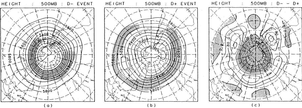
Fig. 4. Synoptic charts projected on a stereographic grid (poleward from 15°S is shown) of the geopotential height field made from 10 case composite for (a) D- events, (b) D+ events (contour interval 100 m) and (c) difference between D- and D+ events (contour interval 40 m). Regions over 20 ms -1 of the u -wind are shaded in (a) and (b). Negative values are shaded in (c).
