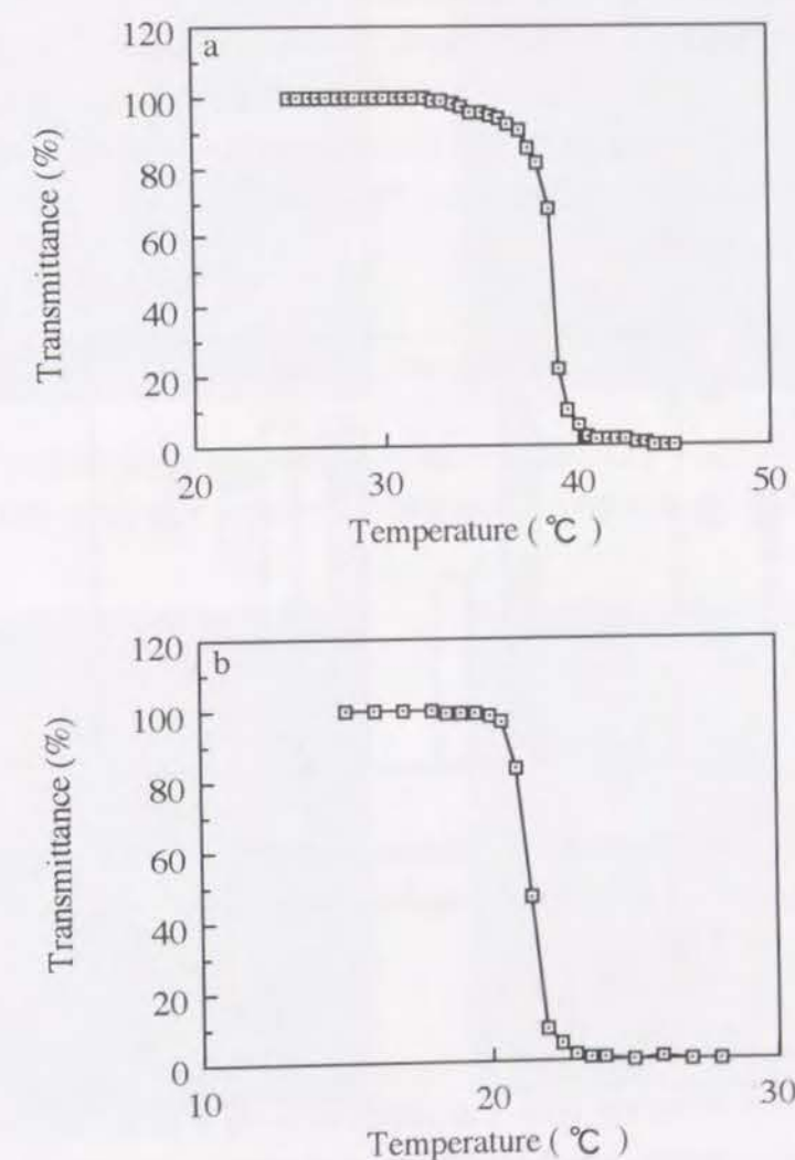
Figure 3 Temperature dependence of turbidity of an aqueous solution of (a) PIA copolymer and (b) azidophenyl-derivatized PIA copolymer.
