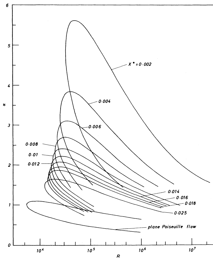
Fig.4. \alpha -R curves for inlet flow profiles.
