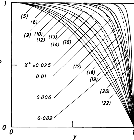
Fig.2. Mean velocity profiles: —, J-H III-1; ----, inlet flow.
