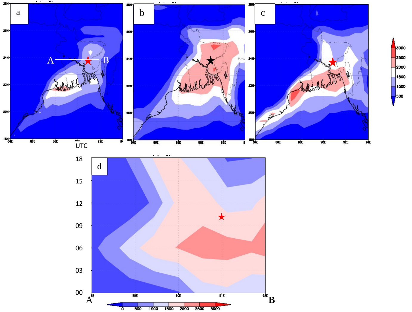
Fig. 8: Shaded CAPE (J/kg) distribution over Bangladesh at (a) 0000 UTC and (b) 0600 UTC (c) 1200 UTC and (d) time series at the cross section of 24°N latitude (A-B line as 8a) from 0000 UTC - 1800 UTC on 22 March 2013 by JRA-55 reanalysis data
