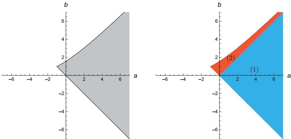
Figure 1. Stability region for (E_1) with \tau = 1 .
