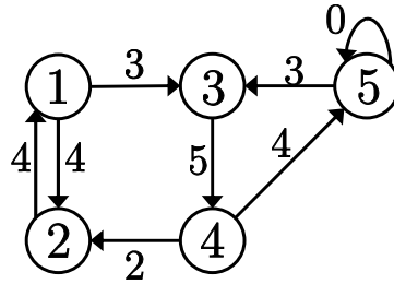
Figure 2. Associated graph \mathcal{G}(A) for Example 3.9.
