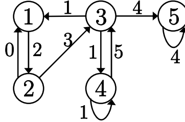
Figure 1. Associated graph \mathcal{G}(A) for Example 2.4.
