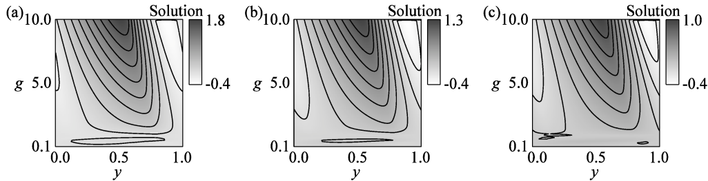
Figure 4: Steady solutions in the bounded case for p=5 and the trend 0.1 \leq g \leq 10 with (a) w_M = 5 , (b) w_M = 6 , and (c) w_M = 7 . The contours correspond to the ten-section lines of the maximum and minimum values.
