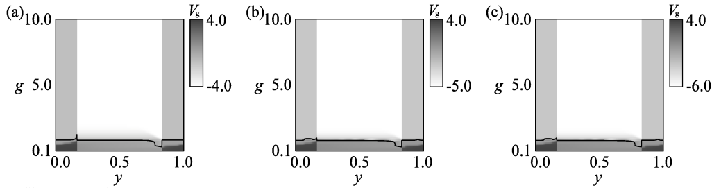
Figure 5: The optimal ground speed in the bounded case for p=2 and the trend 0.1 \leq g \leq 10 with (a) w_M = 5 , (b) w_M = 6 , and (c) w_M = 7 . The black lines correspond to the contour line for V_g = 0 .
