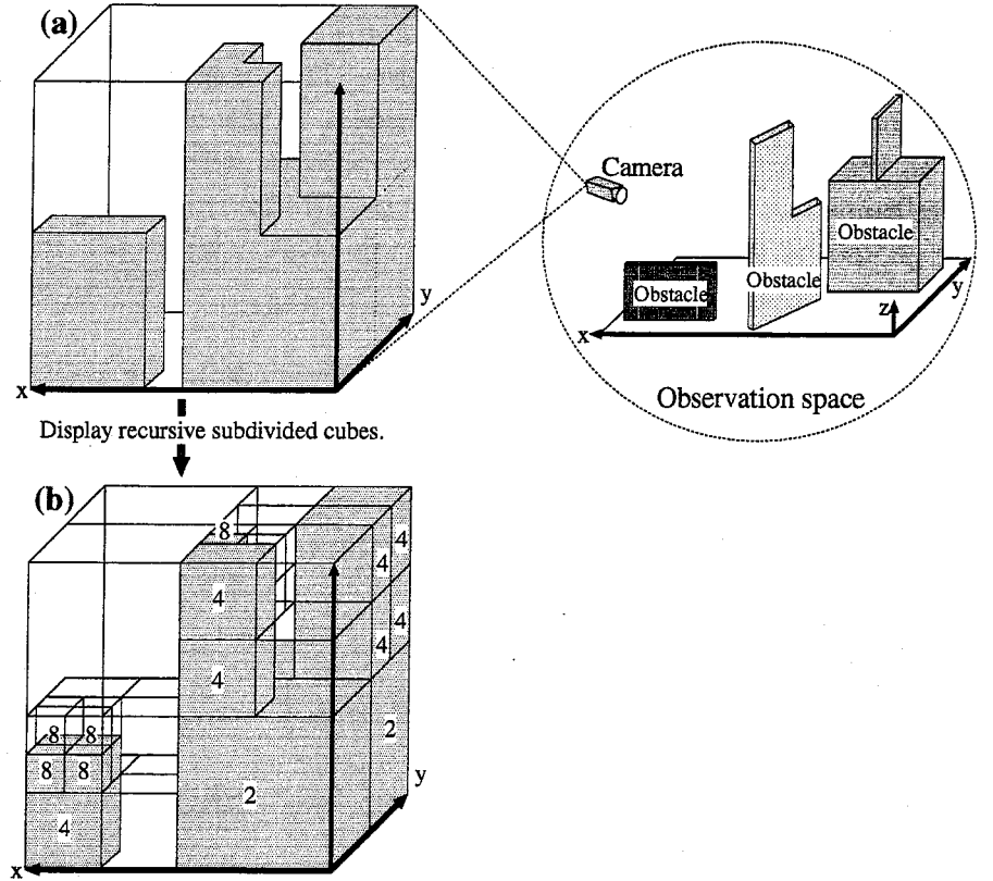
Figure 6.2: Data structure of the observable-area model.
