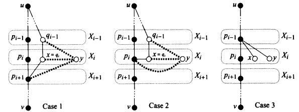
Figure 3: The cases in the proof of Lemma 4.6.
