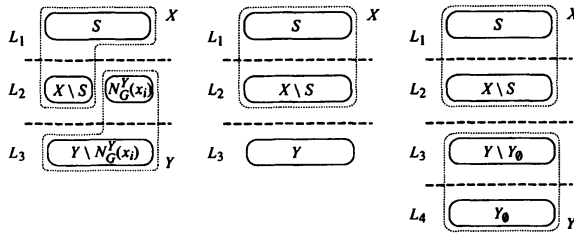
Figure 5: Three cases in the proof of Theorem 5.2.
