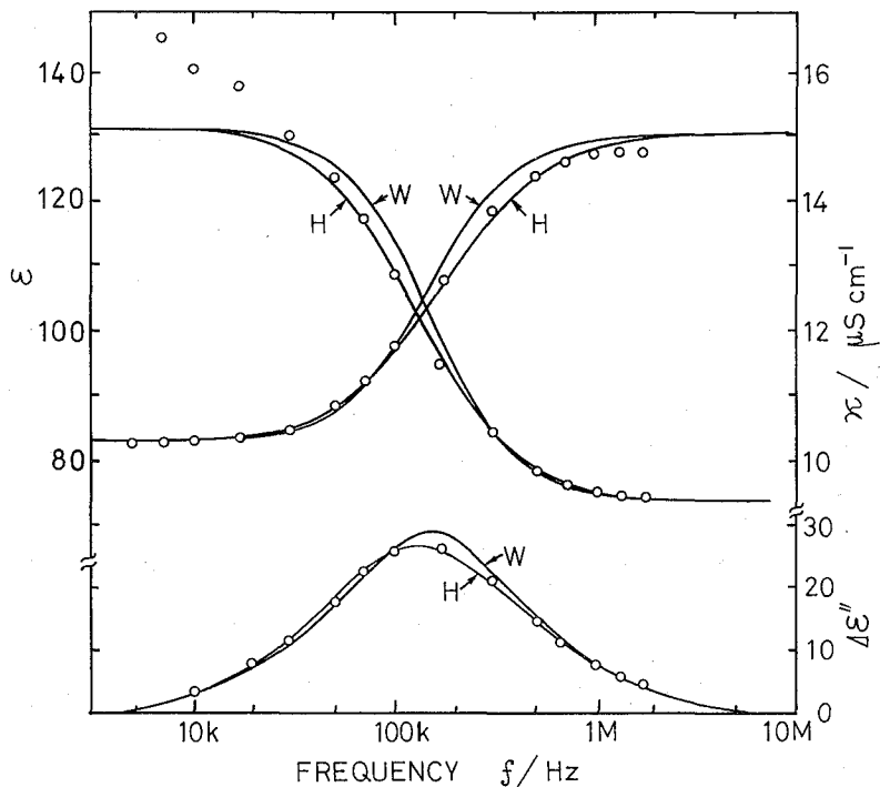
Fig. 3. Frequency dependence of the relative permittivity \epsilon , the electrical conductivity \kappa and the loss factor \Delta\epsilon'' = (\kappa - \kappa_l) / (2\pi f \epsilon_v) for a Sephadex G-25 suspension. The theoretical curves W were calculated from Wagner's Eq. 4, and the curves H from Hanai's Eq. 10.
