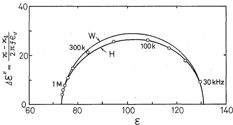
Fig. 4. Complex plane plots of \epsilon and \Delta\epsilon'' for the Sephadex G-25 suspension. The same data as shown in Fig. 3. Curve W was calculated from Wagner's Eq. 4, and curve H from Hanai's Eq. 10. Numbers beside the observed points are the measuring frequency.
