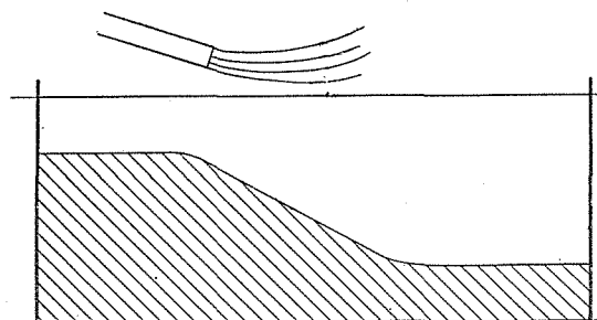
Boundary-Wave Formed by Local Air-Current (cf. Sandström)
