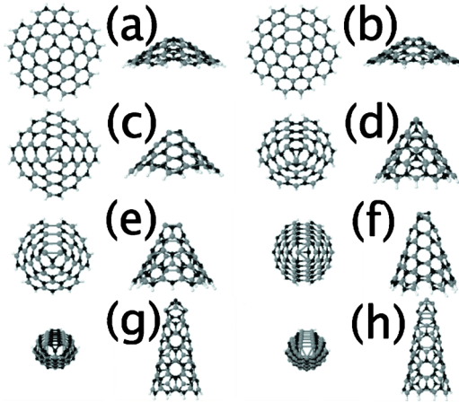
FIG. 1. (Color online) Top and side view of SiCNCs with disclination angles of (a) 60° (C-rich), (b) 60° (Si-rich), (c) 120°, (d) 180° (C-rich), (e) 180° (Si-rich), (f) 240° (C-rich), and (g) 300° (C-rich), and (h) 300° (Si-rich). C-atoms are black, Si-atoms gray, and H-atoms white.
