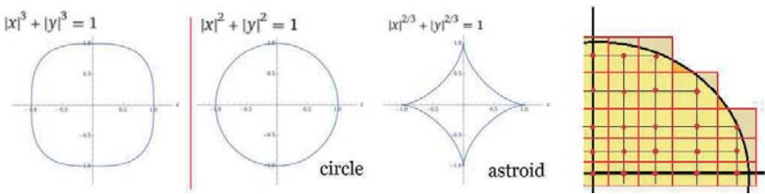
Figure 1: Examples of the p -circle and the approximation by unit squares.
