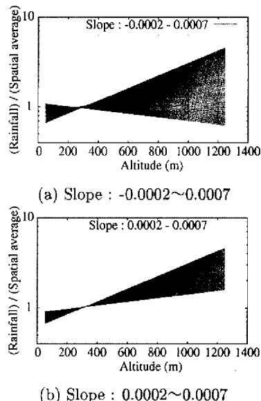
Fig. 7 Sensitivity analysis of regression line depending on topographic altitude
