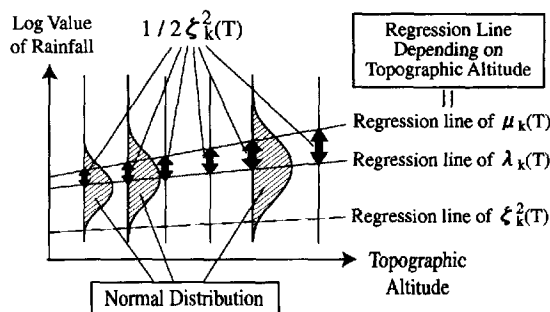
Fig. 17 Schematic diagram of rainfall distribution characteristics (R.A.R > 200mm)
