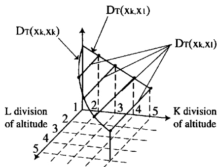
Fig. 22 Modeling of decorrelation distance
