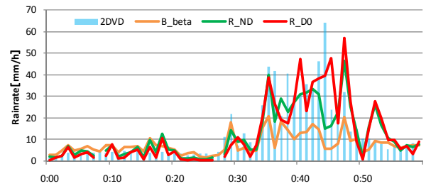
Fig. 8 A time series of rainrate compared with the ground rain gauge.
