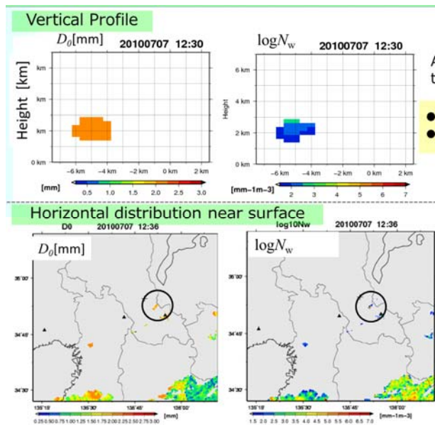
Fig. 6 DSD estimation at heavy rainfall case.
