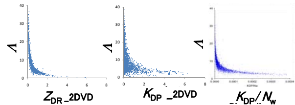
Fig. 3 The relationship between DSD parameter and Polarimetric parameters using 2-dimensional video disdrometer.
