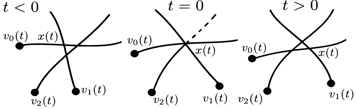
Figure 5. The example found by Aoki-Koike-Takei.
