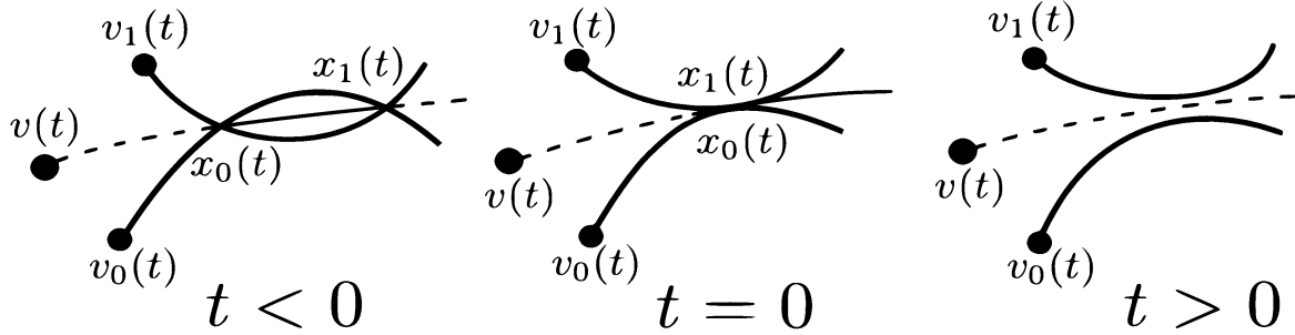
Figure 4. Apply the algorithm to Stokes curves.
