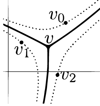
Figure 10. 6 Stokes curves emanating from branches when t \neq t_0
