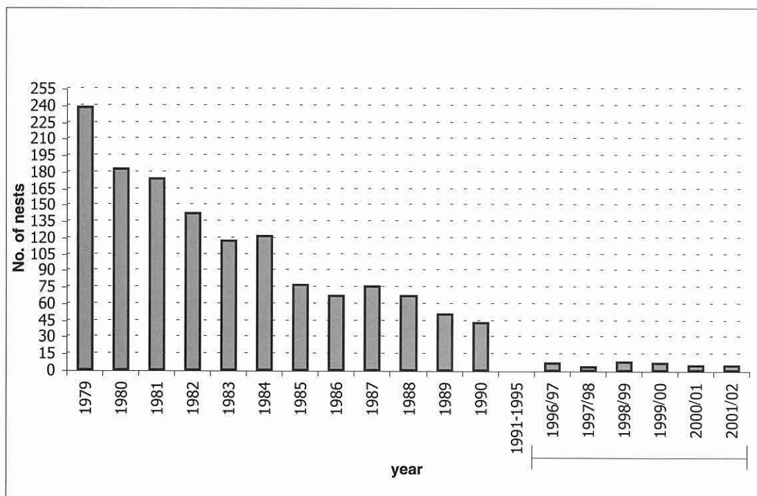
Fig. 2 Olive ridley nests at Phra Thong Island 1979 - 1990
