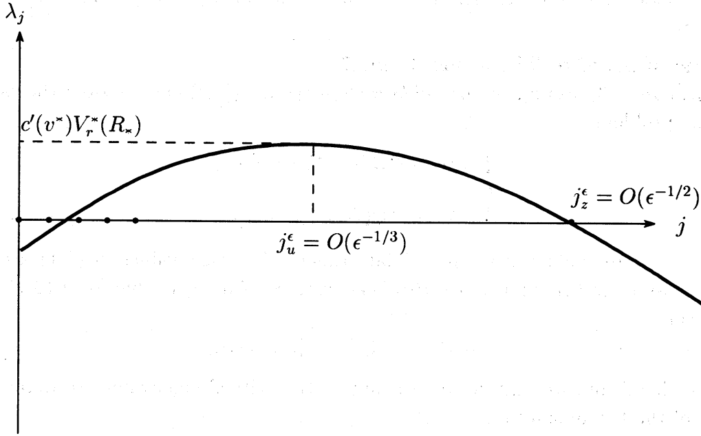
FIGURE 5. Eigenvalues for (AI).
