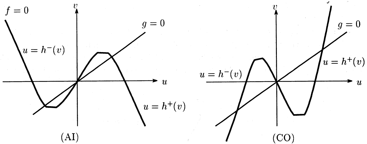
FIGURE 1. Nullclines of (f, g) for (AI) and (CO)
