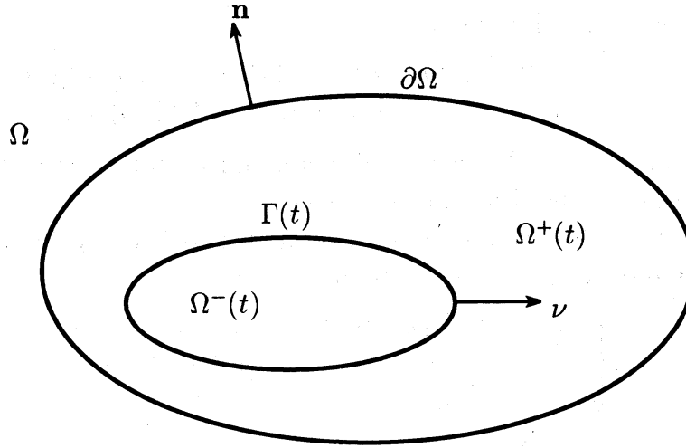
FIGURE 3. \Gamma(t) divides \Omega into two parts, \Omega^-(t) and \Omega^+(t) .
