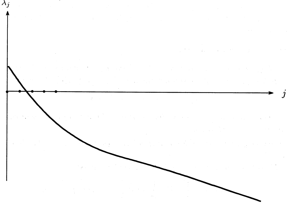
FIGURE 4. Eigenvalues for (CO).
