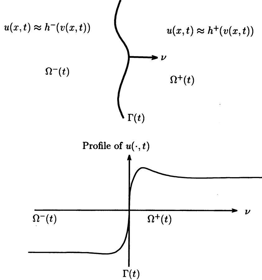
FIGURE 2. Development of interface
