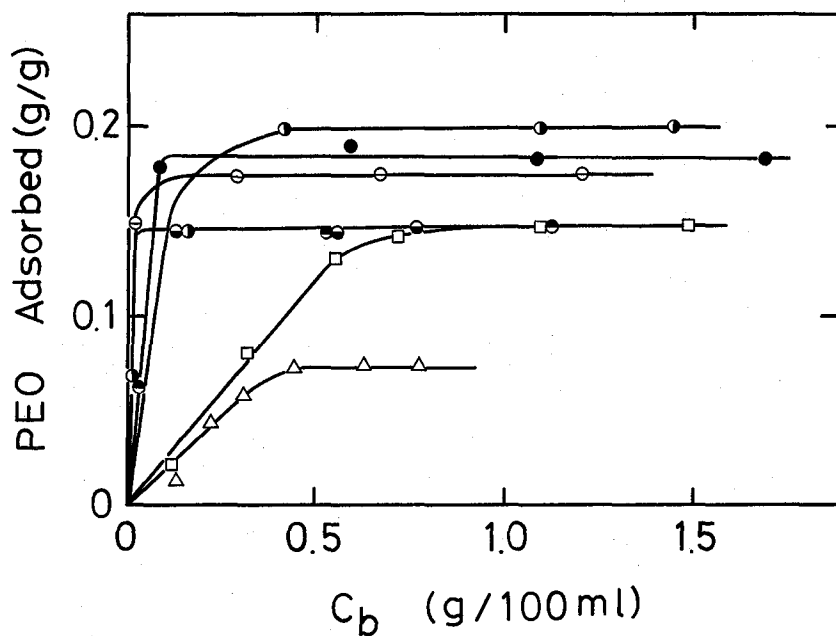
Figure 2. Isotherms for the adsorption of PEO 400, \Delta ; PEO 6,000, \square ; PEO 20,000, \circ ; PEO 86,000, \bullet ; 145,000, \odot ; PEO 594,000, \bullet ; PEO 996,000, \bullet on Ca montmorillonite at 25°C.
