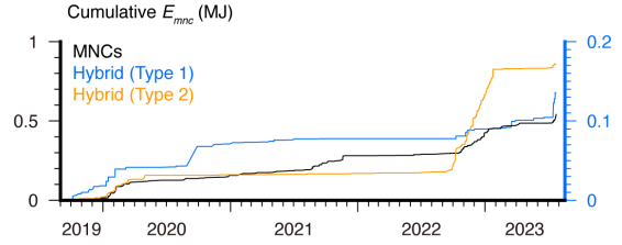
Fig. 8 Time series of cumulative E_{mnc} of MNCs (black), blue (Hybrid Type 1), and orange (Hybrid Type 2). Since the E_{mnc} of Hybrid Type 1 is considerably smaller than the other two types, another vertical scale is set for Hybrid Type 1 (right side with blue color).
