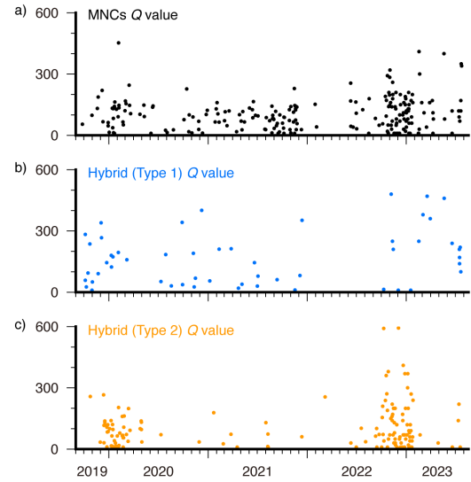
Fig. 13 Time series of quality factor Q of (a) MNCs, (b) Hybrid MNCs (Type 1), and (c) Hybrid MNCs (Type 2).
