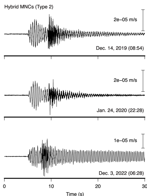
Fig. 5 Examples of the vertical raw ground velocity records of the Hybrid MNCs (Type 2) at FDKL.
