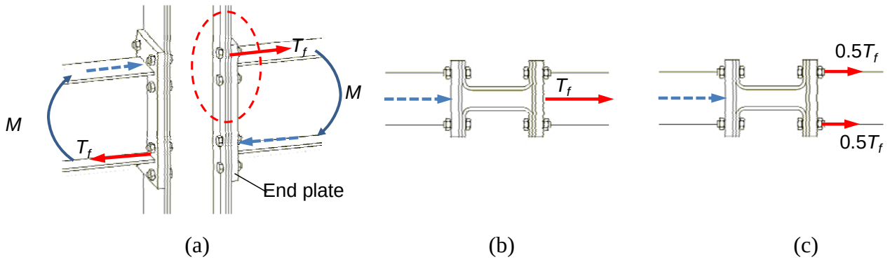
Figure 7.1 Forces on the column flanges in the beam-to-column connection: (a) forces from the beam flanges; (b) view from top; (c) applied force divided into two halves.
