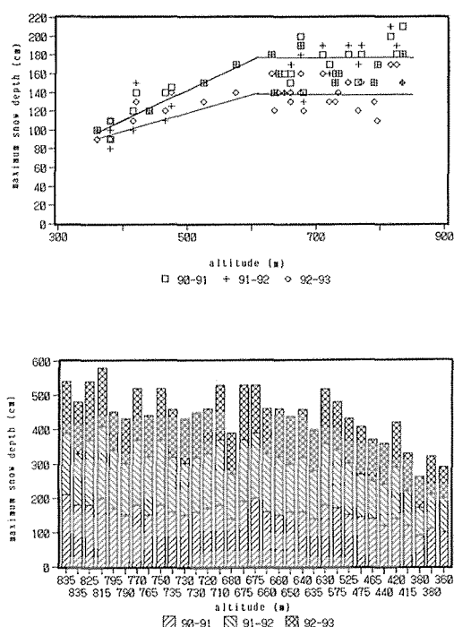
図13 最大積雪深と標高の関係 Relationship between maximum snow depth and altitude
