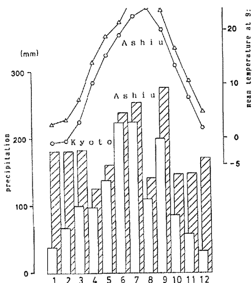
図9 芦生演習林の降水量と気温 Precipitation and temperature in Ashiu
