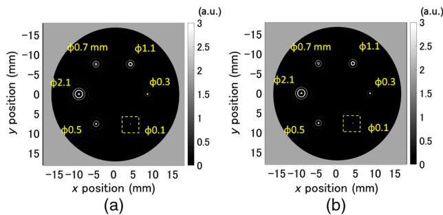
Fig. 6 Reconstructed images in each element width. The center frequency and fractional bandwidth used in the calculation were 3 MHz and 80%, respectively. (a) A result calculated by infinitesimal elements. (b) A result calculated by averaging 20 infinitesimal elements. Each 0.1-mm-diameter blood vessel is marked by a yellow-dotted square as shown in Fig. 7.
