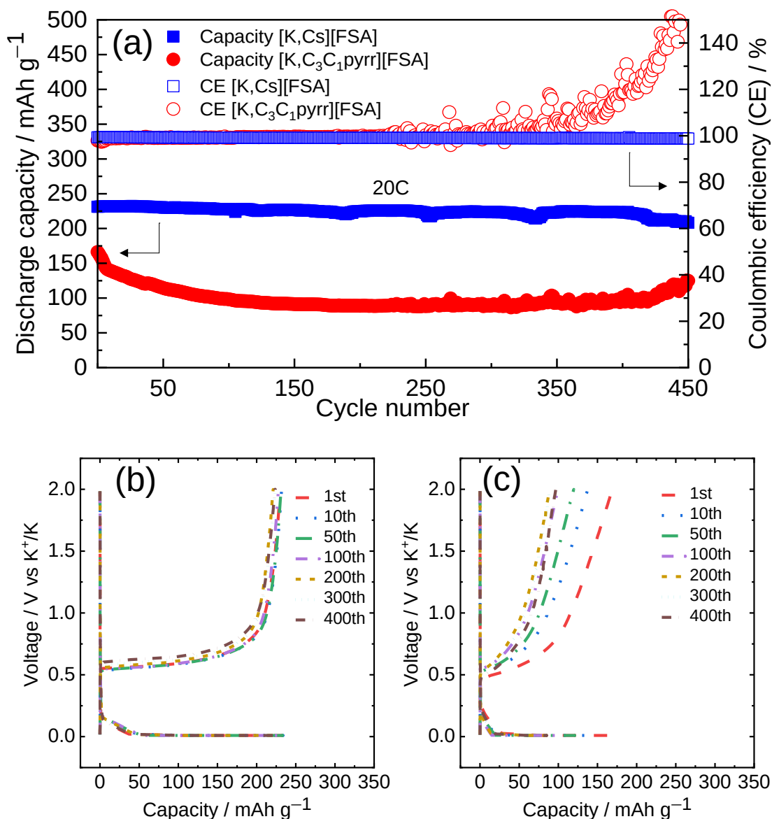
Figure 4. (a) Cycle performance of K/graphite half-cells (graphite average particle size = 10 \mu\text{m} ) employing the [\text{K,Cs}][\text{FSA}] IL and [\text{K,C}_3\text{C}_1\text{pyrr}][\text{FSA}] IL electrolytes. Charge-discharge curves obtained during the cycle performance tests on cells with the (b) [\text{K,Cs}][\text{FSA}] IL and (c) [\text{K,C}_3\text{C}_1\text{pyrr}][\text{FSA}] IL electrolytes. Current density = 20C (additional constant voltage charge at 0.01 V), cut-off voltage = 0.01–2.0 V. [\text{K,Cs}][\text{FSA}] = \text{K}[\text{FSA}]\text{-Cs}[\text{FSA}] IL (54 : 46 in mol) and [\text{K,C}_3\text{C}_1\text{pyrr}][\text{FSA}] = \text{K}[\text{FSA}]\text{-C}_3\text{C}_1\text{pyrr}[\text{FSA}] IL (20 : 80 in mol). The cycle tests presented here were performed after the rate capability tests.
