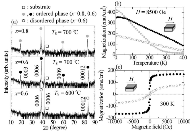
FIG. 1. (a) XRD patterns of x\text{FeTiO}_3\cdot(1-x)\text{Fe}_2\text{O}_3 [ x=0.6 (filled circles) and 0.8 (gray circles)] solid-solution thin films prepared under the optimized deposition conditions to obtain the ordered phase ( P_{\text{O}_2} of 2.0\times 10^{-3} Pa and T_s of 700^\circ\text{C} ) along with the pattern of 0.6\text{FeTiO}_3\cdot 0.4\text{Fe}_2\text{O}_3 solid-solution thin film prepared at T_s of 600^\circ\text{C} (open circles). (b) Temperature dependence of magnetization of each film. (c) Magnetic field dependence of magnetization at 300 K.
