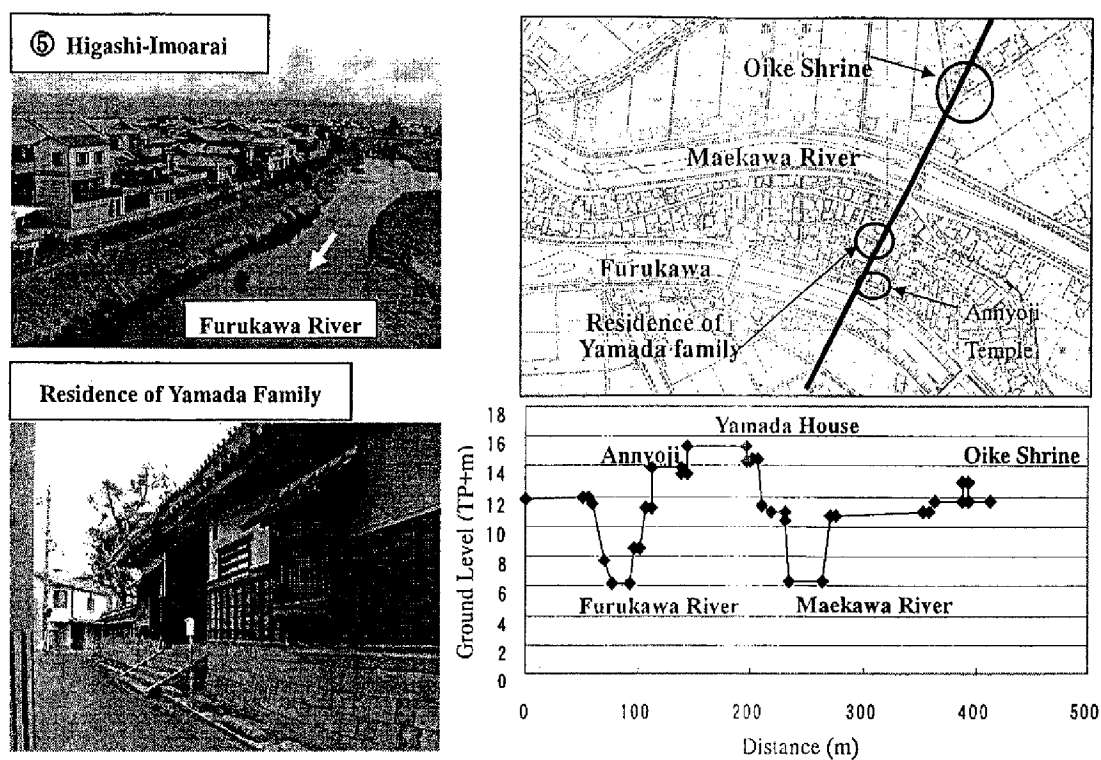
Fig.2 Old houses with raised base in Higashi-Imoarai and the cross-section of this area.
