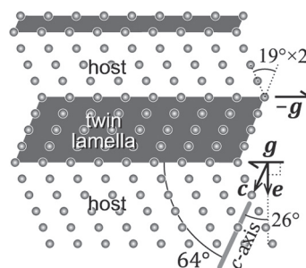
Fig. 5. Geometry of e -twinning in calcite. Gray balls represent calcite atoms. The twinning results in simple shear along the twin lamella. See text for the definitions of vectors.
