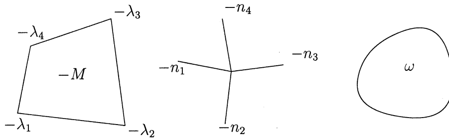
図 1: -M , \text{Char}(S*)^a and \omega
