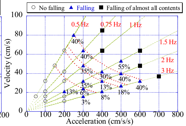
Fig. 12 Test results of the powder medicine shelf subjected to sinusoidal waves (Specimen 9, H180-W180-B15-60)
