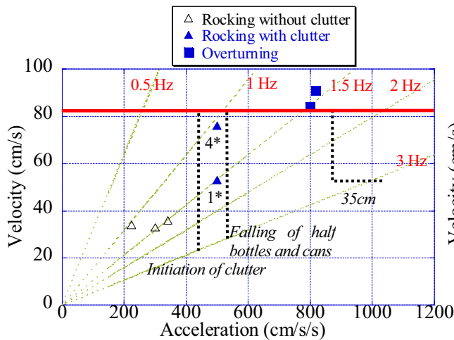
Fig. 15 Test results of the tablet medicine shelf subjected to earthquake motions (Specimen 7)
