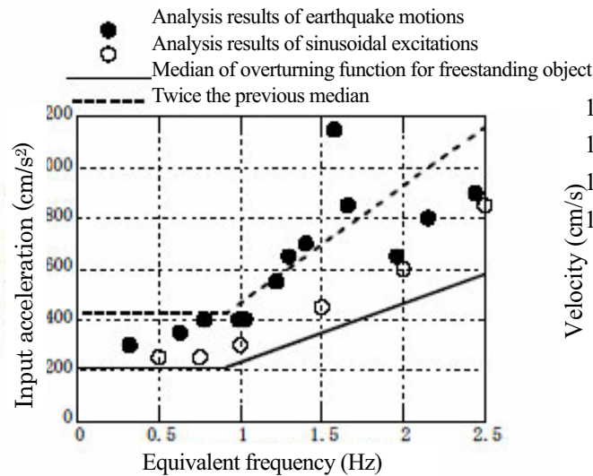
Fig. 13 Comparison of overturning accelerations under sinusoidal waves and earthquakes (Tamura et al. 2005)
