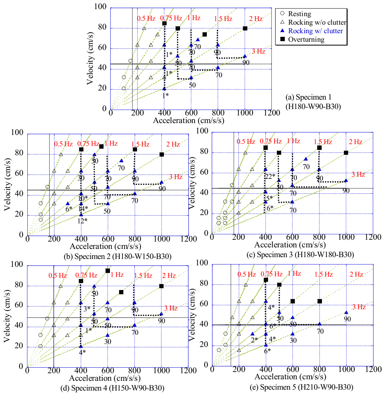
Fig. 10 Test results of the stock shelf subjected to sinusoidal waves (* denotes the number of fallen items)
