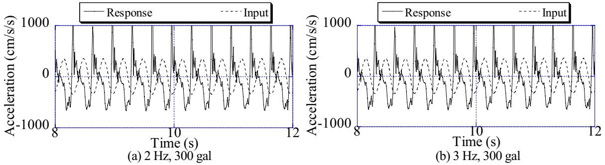
Fig. 9 Amplification of acceleration at the top of the powder medicine shelf (Specimen 9) subjected to sinusoidal waves
