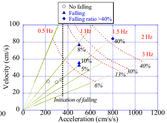
Fig. 16 Test results of the powder medicine shelf subjected to earthquake motions (Specimen 9)
