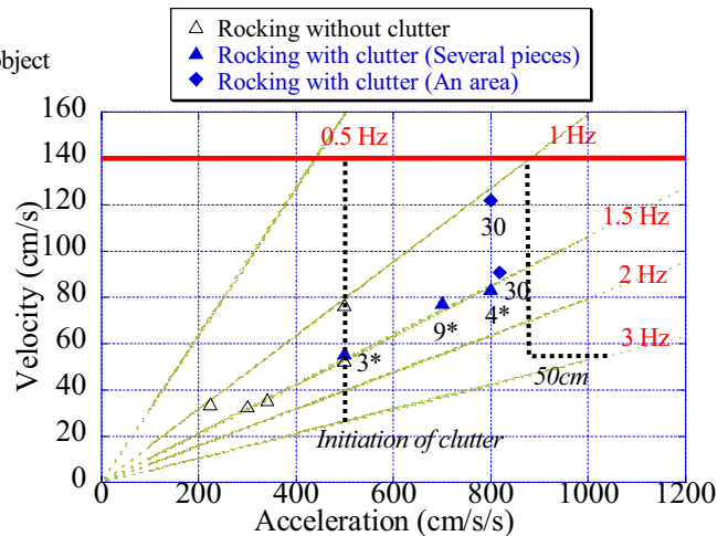
Fig. 14 Test results of the stock shelf subjected to earthquake motions (Specimen 2)
