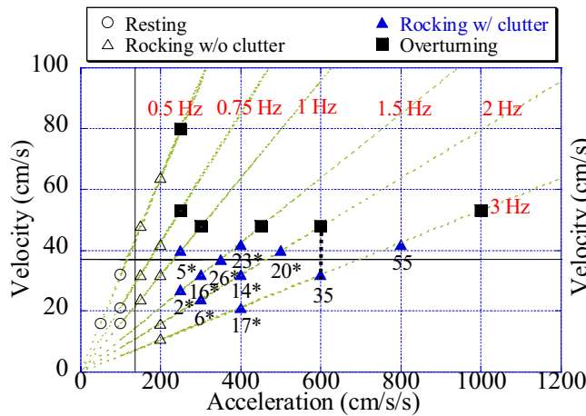
Fig. 11 Test results of the tablet medicine shelf subjected to sinusoidal waves (Specimen 8, H180-W180-B25; * denotes the number of fallen items)
