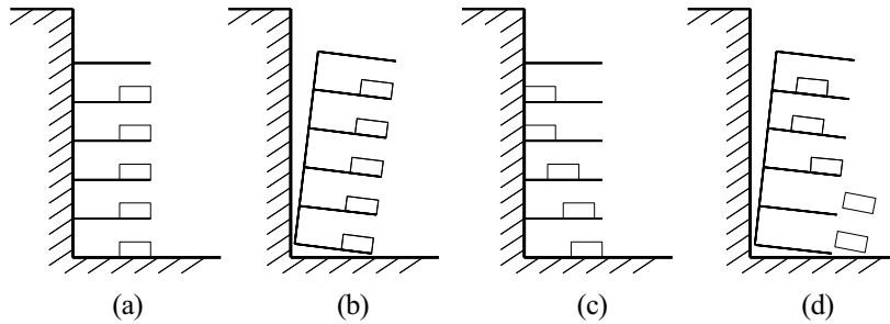
Fig. 5 Motions of the stock shelf and falling of medicine packages
