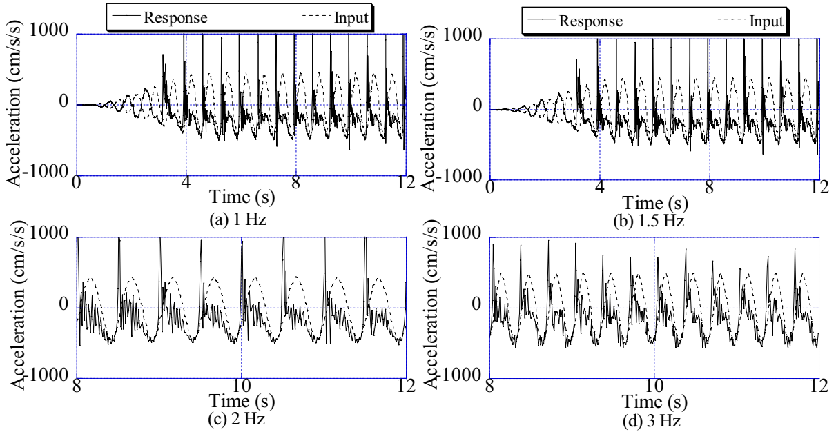
Fig. 6 Response at the top of the stock shelf (Specimen 1) under sinusoidal waves of 400 gal peak acceleration
