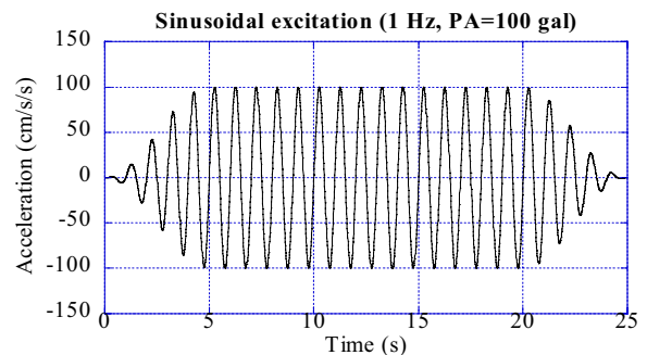
Fig. 3 Input of sinusoidal wave
