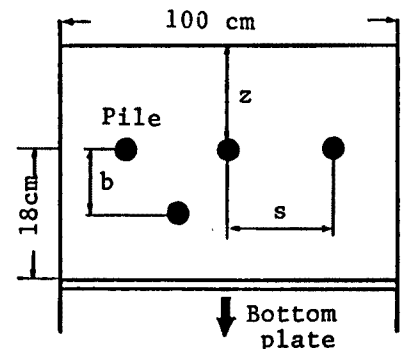
Fig. 9 Pile space and overburden length.
