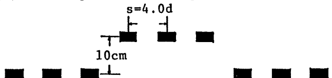
Fig. 8 Arrangement of landslide prevention piles.
