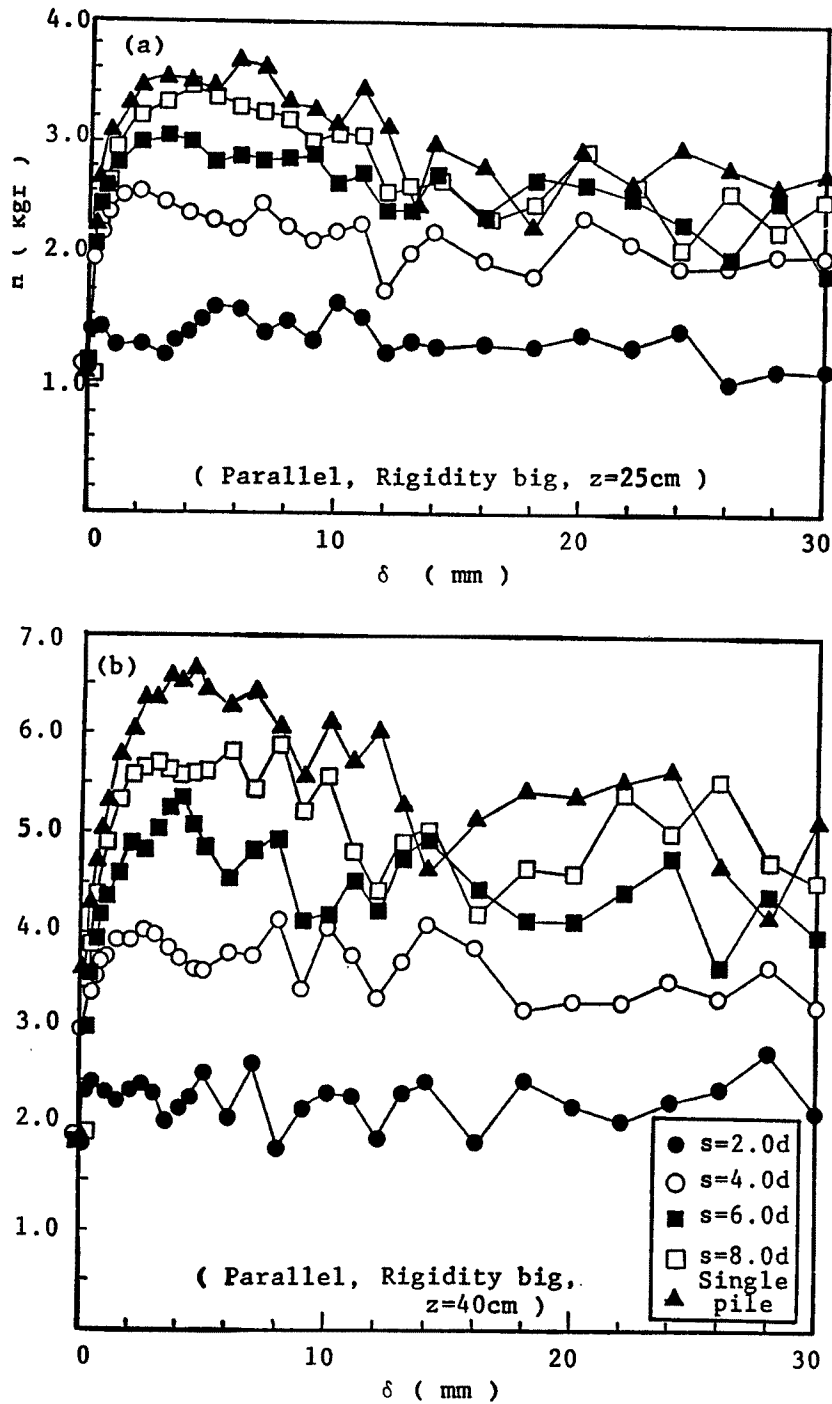
Fig. 17 Effect of overburden length. ((a) z=25\text{ cm} , (b) z=40\text{ cm} )
