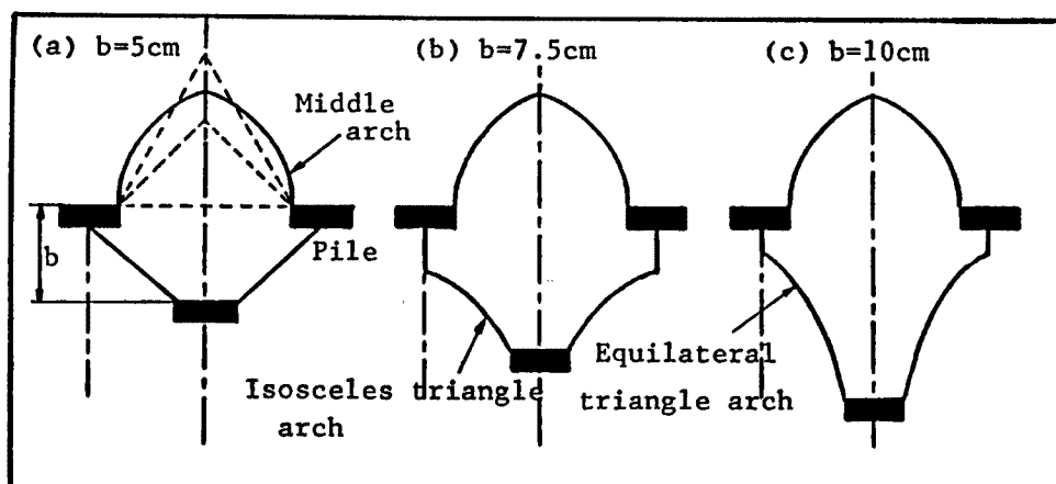
Fig. 24 Shape of arch for zigzag arrangement.
