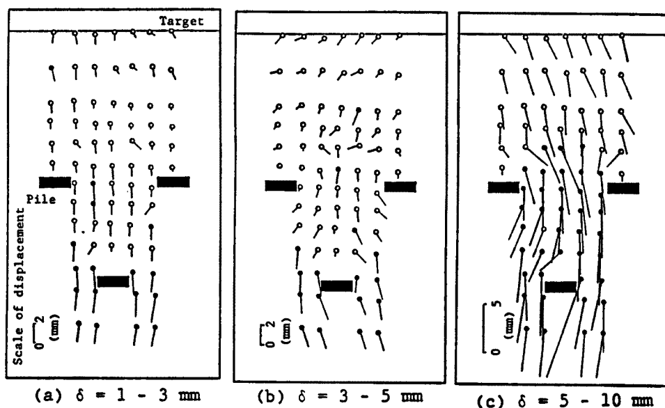
Fig. 23 Displacement vector of targets. (Zigzag arrangement, s=2.0 d, z=15 cm, b=10 cm)
