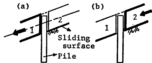
1,2;Landslide mass
