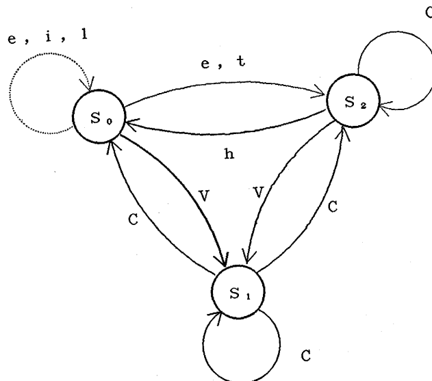
Fig. 2(d). Representative transitions in the 3-state HMM for English.
