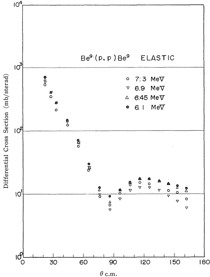
Fig. 5. The angular distributions of the elastic scattering of protons by \text{Be}^9 at 7.3~6.1 Mev proton energies.
