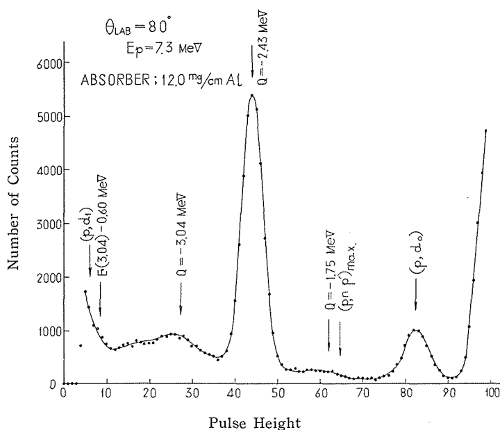
Fig. 3. Typical pulse height spectrum obtained with the absorber before the detector. The relative position of (p, d_1) is shifted markedly.
