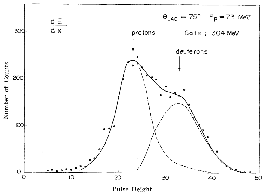
Fig. 2. The dE/dx spectra for the scattered particles comprised in the section of the pulse spectrum corresponding to the 3.04 Mev group and the 2.43 Mev group.
