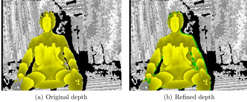
Figure 3.7: Depth correction.
