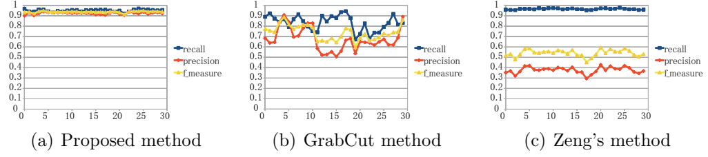
Figure 2.14: Evaluation values in each camera viewpoint (Sequence B).
