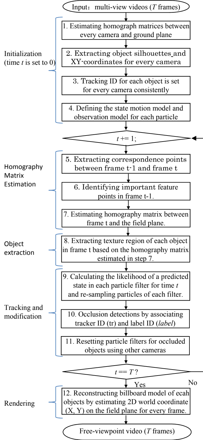
Figure 4.1: Flowchart of the proposed method.
