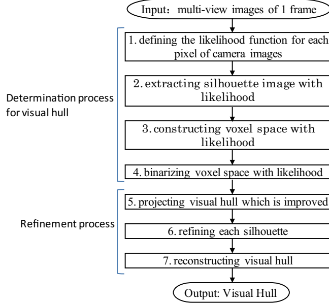
Figure 2.1: Flow chart of proposed method.
