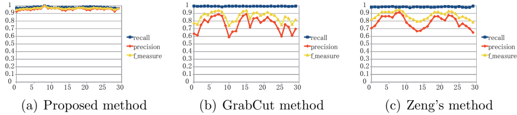
Figure 2.13: Evaluation values in each camera viewpoint (Sequence A).
