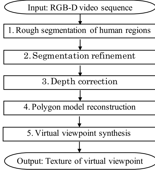
Figure 3.4: Flowchart of the proposed method.
