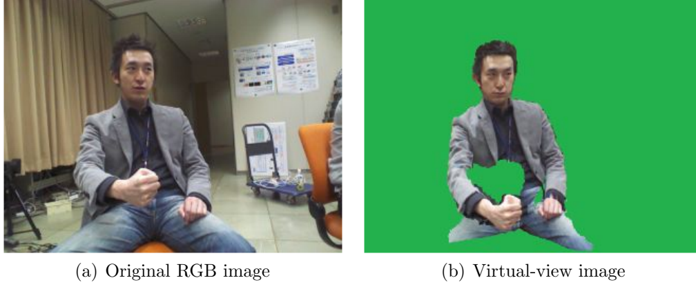
Figure 3.9: Dis-occlusion detection.
