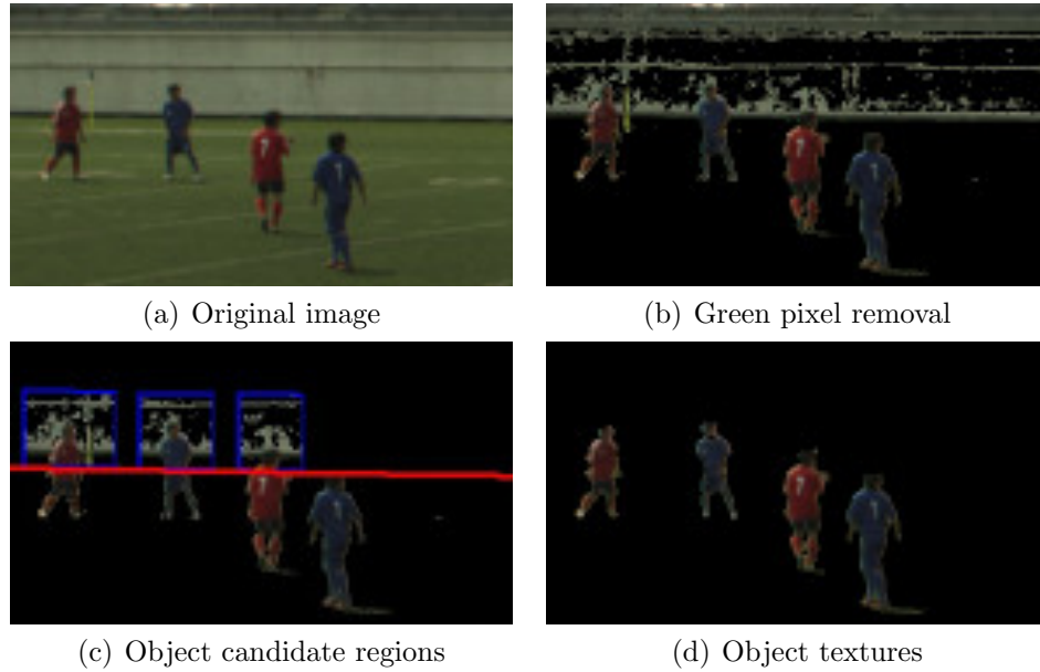
Figure 4.8: Examples of extracted object textures.
