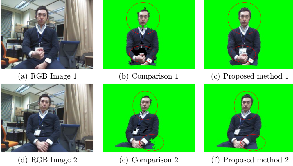
Figure 3.20: Synthesized virtual viewpoint images.
