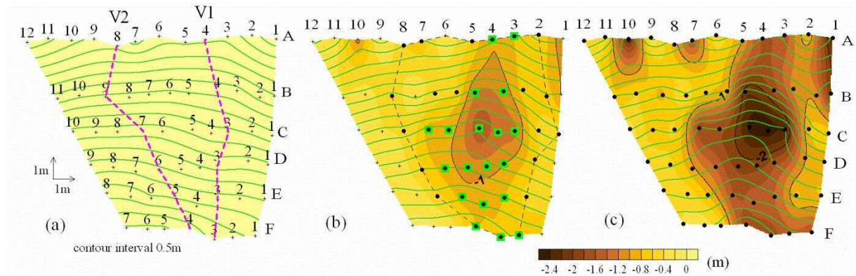
Fig. 4.1 (a) Ground surface topographic map and locations of all observation points. The broken line indicates the location of the vertical cross-section regarded as Lines-V1 and V2. (b) Middle layer topographic map and soil thickness distribution from ground surface to the middle layer. Dots and squares denote the tensiometers installed in shallow and middle layers, respectively. Tensiometers were not installed in shallow and middle layers outside the domain bounded by the broken line. (c) Bedrock surface topographic map and soil thickness distribution from ground surface to bedrock surface. Dots denote tensiometers installed at the soil-bedrock interface. The contour interval of each topographic map is 0.5 m.
