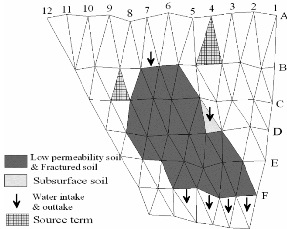
Fig. 4.9 Locations of weathered bedrock layer (low permeability soil and fractured soil), bedrock groundwater seepage area (source term), and water intake/outtake in top view.
