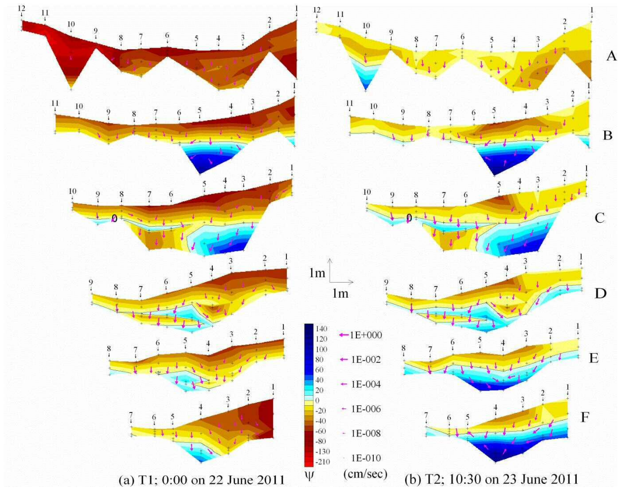
Fig. 4.13 Distributions of calculated pressure head, \psi , in the vertical cross-sections of Lines-A to F at time points (a) T1 and (b) T2. Arrows denote the calculated magnitude and direction of water flux vectors.
