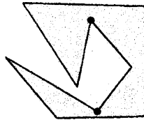
Figure 4: A spiral polygon such (i) the minimum number of guards is two and (ii) a unique set of two guards.
